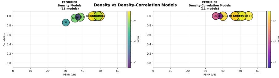
Figure 3: LagrangeBench TGV-2D, Fourier basis: PSNR vs. correlation for 11 architectures. Left: models trained with the MSE objective; right: models trained with the hybrid (MSE + correlation) objective. Each bubble is one model; the x-axis shows PSNR (dB) and the y-axis shows Pearson correlation. Bubble brightness and bubble area is proportional to FLOPs.
