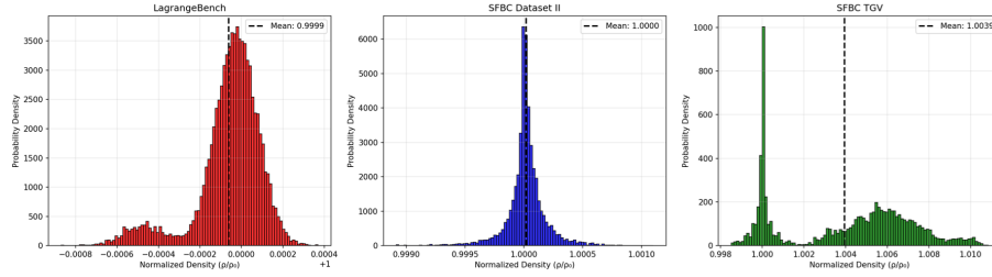
Figure 1: Density distributions \rho normalized on \rho_0 (density at rest) aggregated over all frames for the three datasets. The dashed vertical line marks the mean of each distribution, where all datasets are centered near 1.
