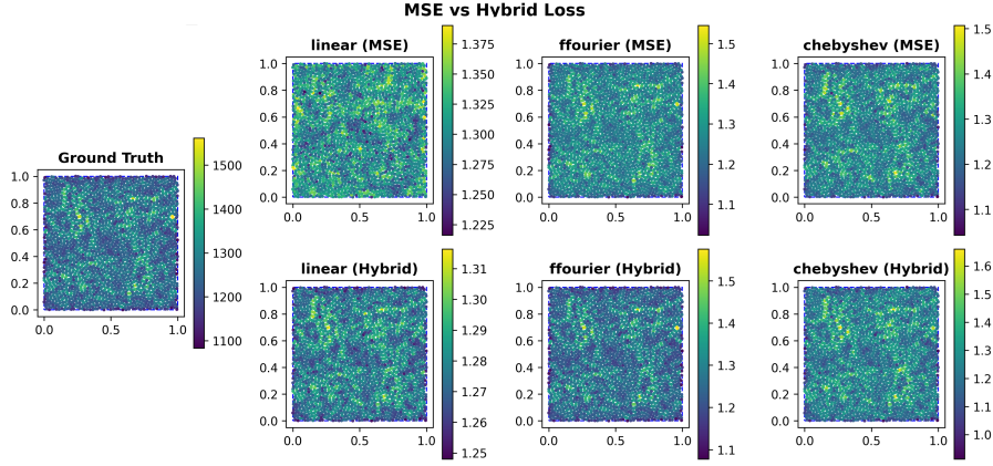
Figure 2: Qualitative comparison of MSE vs. Hybrid loss on LagrangeBench TGV-2D (test trajectory 15, frame 100). Left column shows the ground-truth density; the top row shows predictions from the [32, 16, 1] architecture trained with the plain MSE objective, and the bottom row shows the same architecture trained with the Hybrid objective (MSE + correlation + scale penalty).
